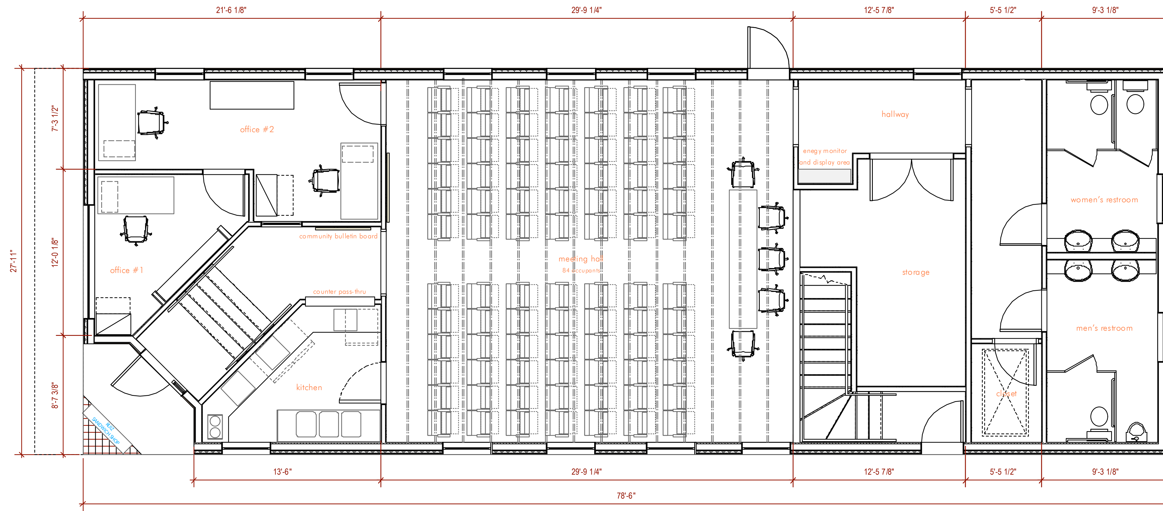
1 First Floor Plan 1/4" = 1'-0"
