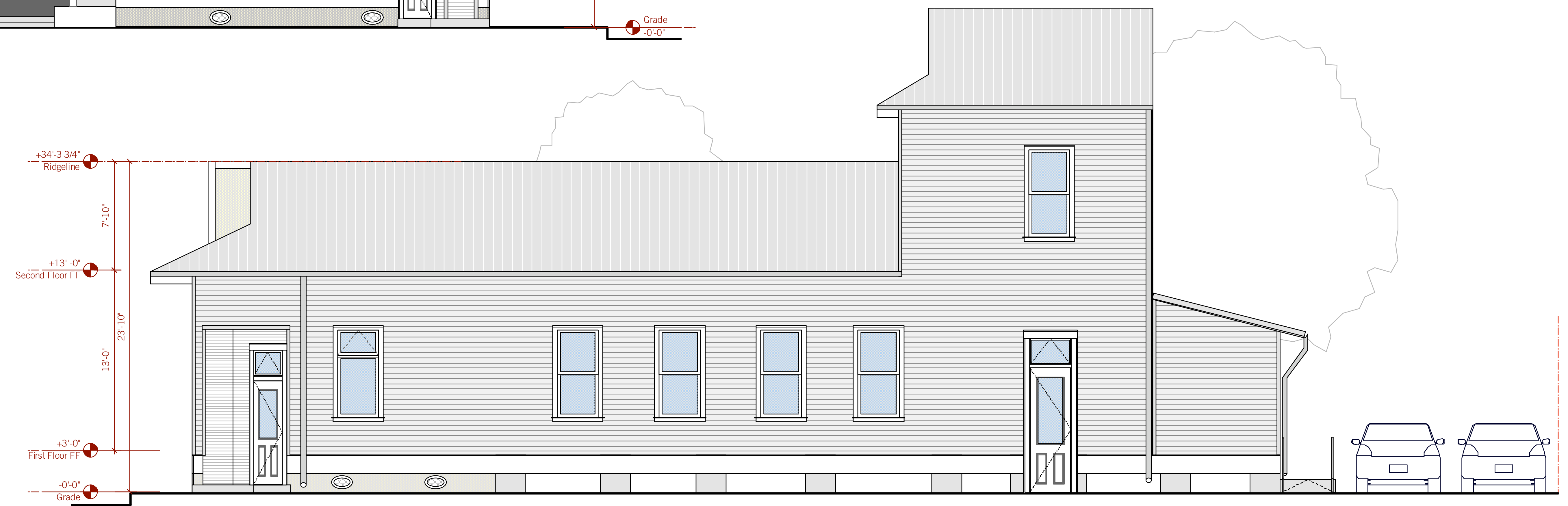
2 Elevation: East [Egania Street Side] 1/4" = 1'-0"
